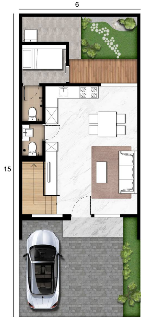
LANTAI 1
